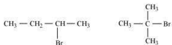
2 - Bromobutane (2°) 2 - Bromo - 2 - methylpropane (3°)
